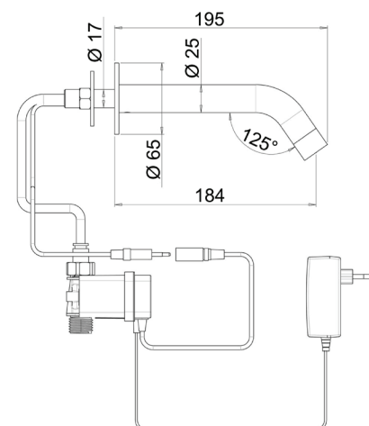
RES-911 panel mounted version, transformer
