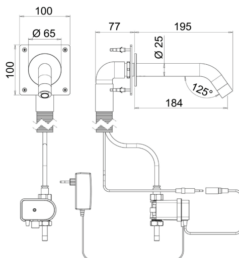
RES-912 recessed version, transformer
