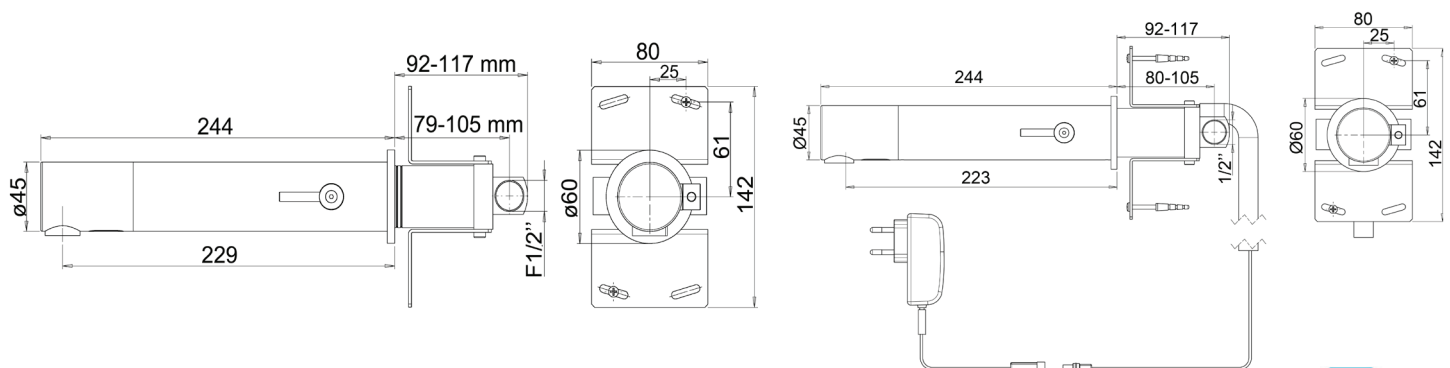
RES-260 recessed version, battery
