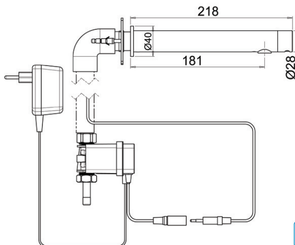
RES-143 recessed version, transformer
