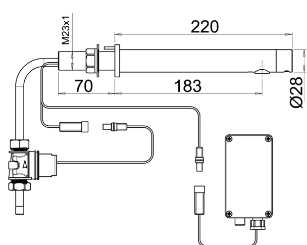
RES-140 panel mounted version, battery
