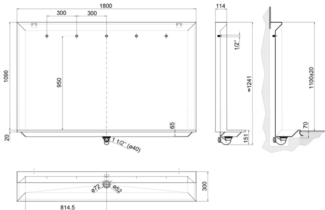
Dimensions IN-S1800
